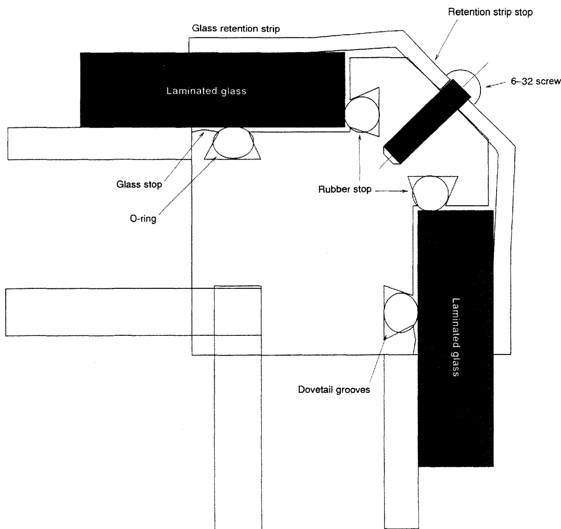
Figure 4.6 Schematic of the hermetic seal.
